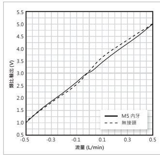
● KFPSA-R005 (-0.5 ~ 0.5 L/min)
