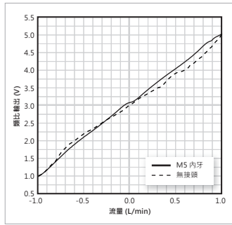
● KFPSA-R010 (-1 ~ 1 L/min)
