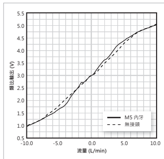
● KFPSA-R100 (-10 ~ 10 L/min)
