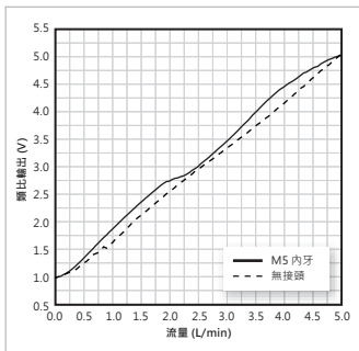
● KFPSA-050 (0 ~ 5 L/min)
