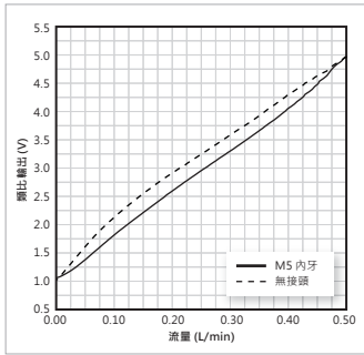
● KFPSA-005 (0 ~ 0.5 L/min)
