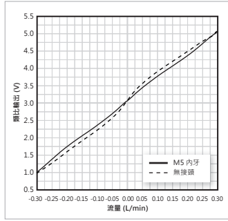
● KFPSA-R003 (-0.3 ~ 0.3 L/min)
