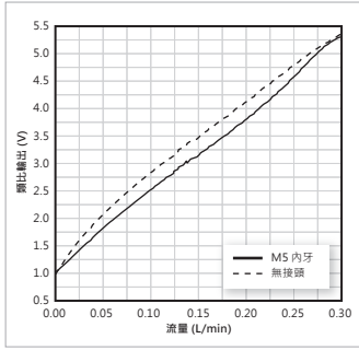
● KFPSA-003 (0 ~ 0.3 L/min)
