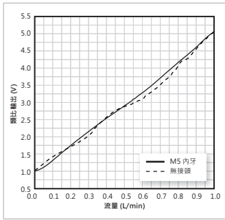
● KFPSA-010 (0 ~ 1 L/min)
