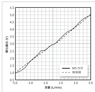
● KFPSA-R050 (-5 ~ 5 L/min)
