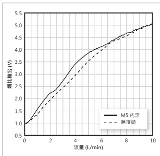
● KFPSA-100 (0 ~ 10 L/min)
